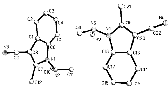
Fig. 2 X-Ray crystallography of 2a .
